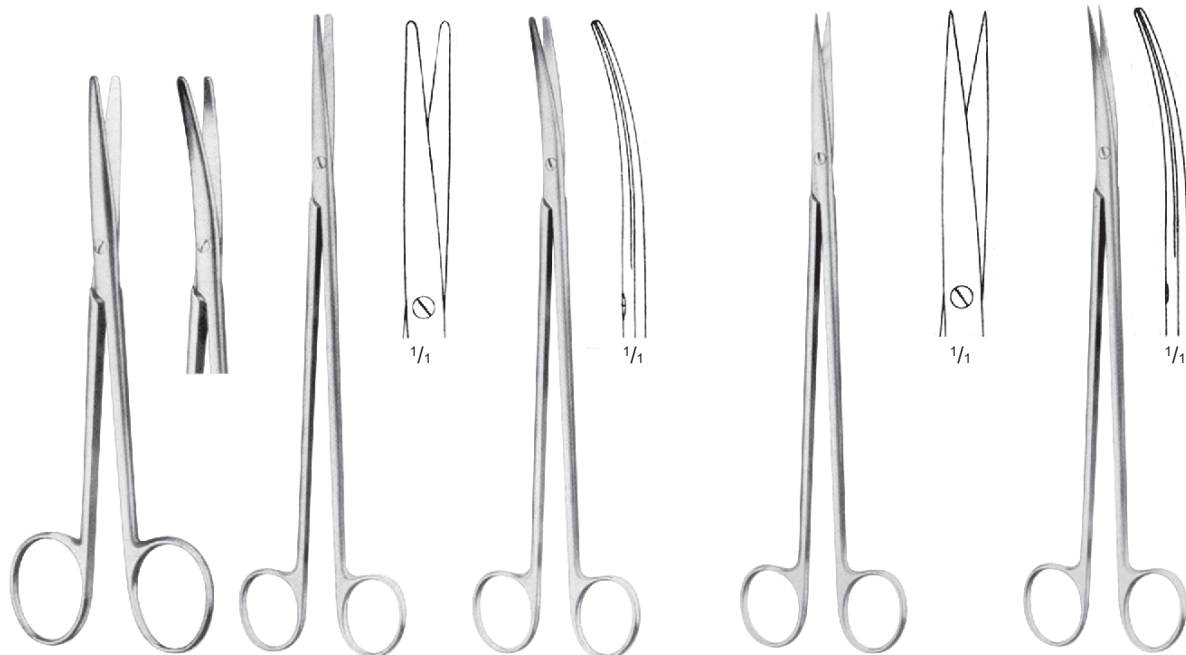
LEXER C-SI3314 = 16 cm / 6 1/2" C-SI3315 = 21 cm / 8 1/2" LEXER C-SI-3316 = 16 cm / 6 1/2" C-SI3317 = 21 cm / 8 1/2" FOMON C-SI3318 13,5 cm / 5 1/4" THOREK C-SI3319 = 19 cm / 7 3/4" C-SI3320 = 25,5 cm / 10" LEXER-BABY C-SI3321 = 10 cm / 4" C-SI3322 = 12 cm / 4 3/4" LEXER-BABY C-SI3323 = 10 cm / 4" C-SI3324 = 12 cm / 4 3/4"
